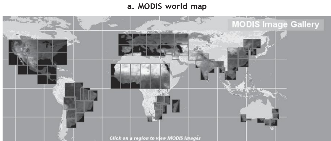
Figure 6.8 MODIS Image Gallery
